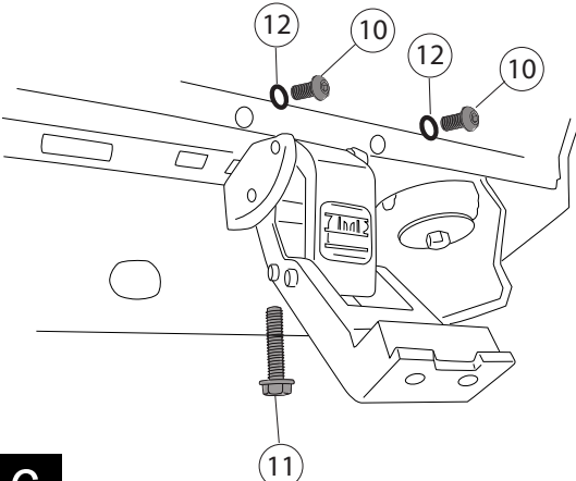
6 Repeat linkage installation on driver side
